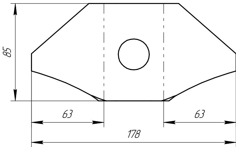
Q (1:2)
